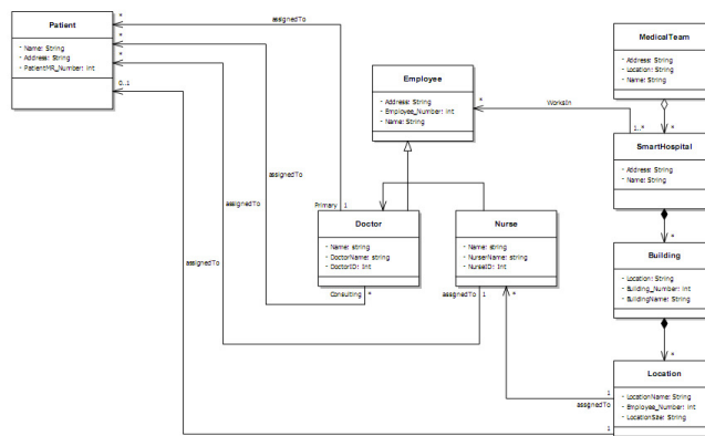
Figure 7(b). Class diagram for asset assignment
