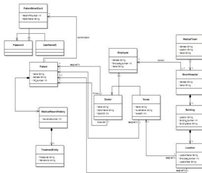
Figure 7(a). Class diagram for patient treatment.
