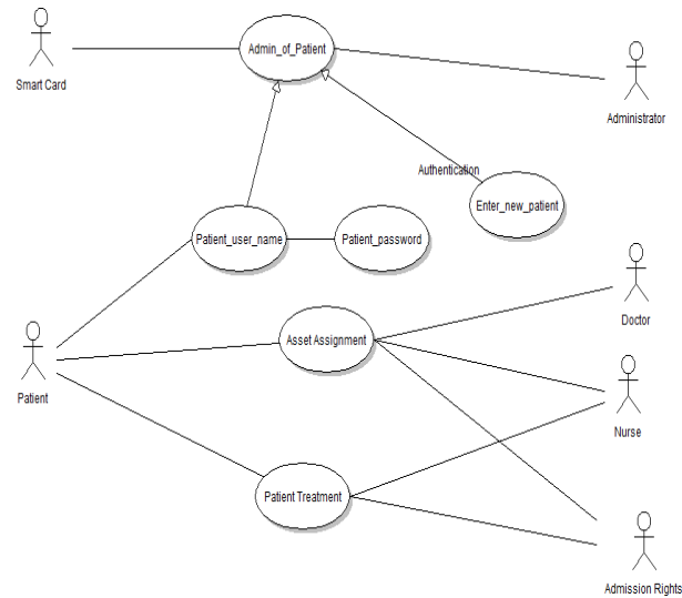
Figure 1a. Use-case diagram
